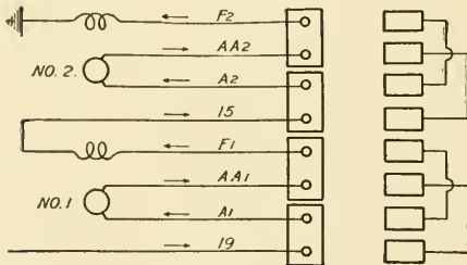
Fig. 56. Reverse Position of Reverse
